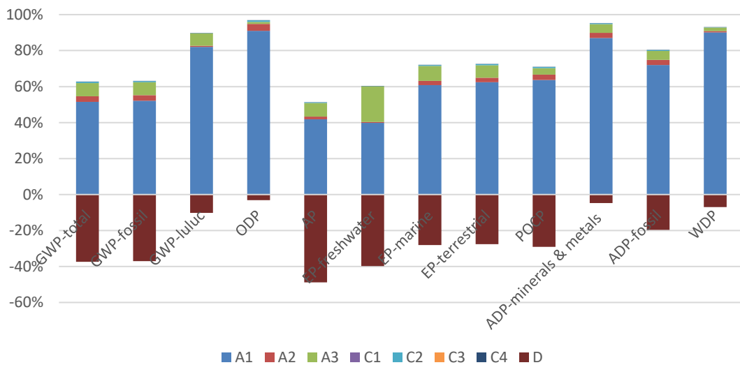
Figure 4. Shares of life cycle modules in the main categories of impacts screw-in facade fixings R-TFIX-8S-X.
